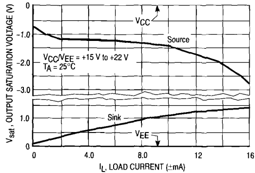
Figure 5. Output Saturation versus Load Current
