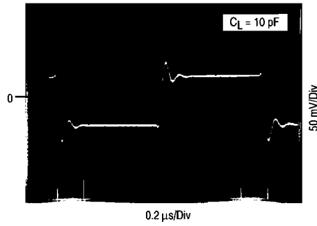
Figure 26. Small-Signal
