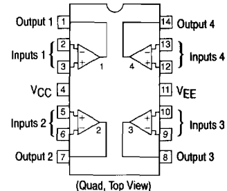
P SUFFIX PLASTIC PACKAGE CASE 646
