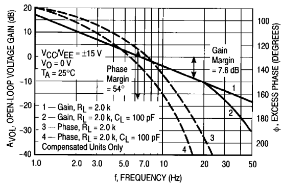
Figure 15. Open-Loop Voltage Gain and Phase versus Frequency
