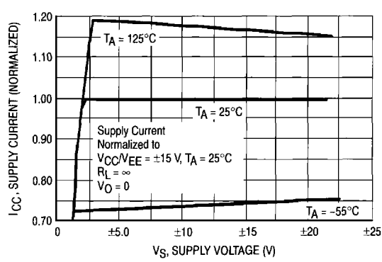
Figure 31. Normalized Supply Current versus Supply Voltage
