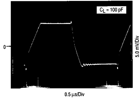
Figure 25. Large-Signal
