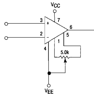
Figure 34. Offset Nulling Circuit
