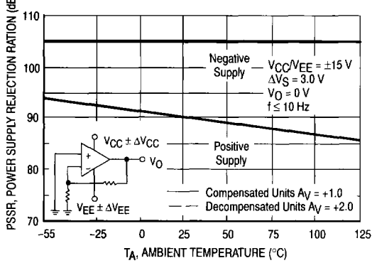
Figure 30. Power Supply Rejection Ratio versus Temperature
