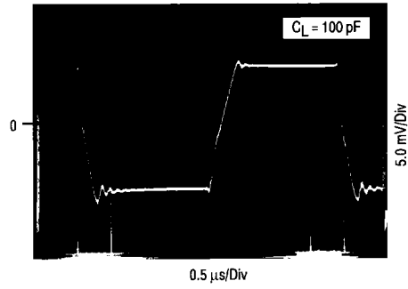
Figure 27. Large-Signal
