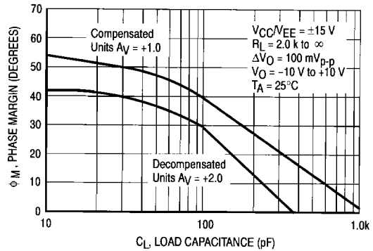
Figure 19. Phase Margin versus Load Capacitance
